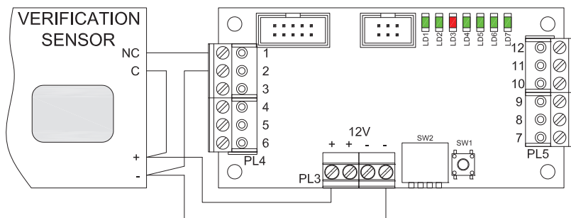
SmokeCloak Easy interface to alarm panel wiring VERIFICATION SENSOR CONNECTION
