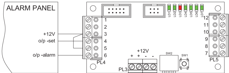
SmokeCloak Easy interface to alarm panel wiring NEGATIVE SET AND NEGATIVE TRIGGER 3256-A
